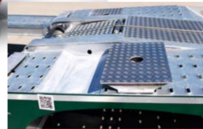
Additional front wheel recesses and covers
